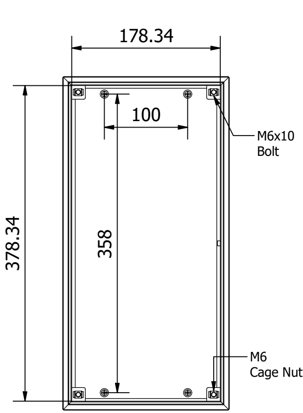
FRONT VIEW (OPENING)
