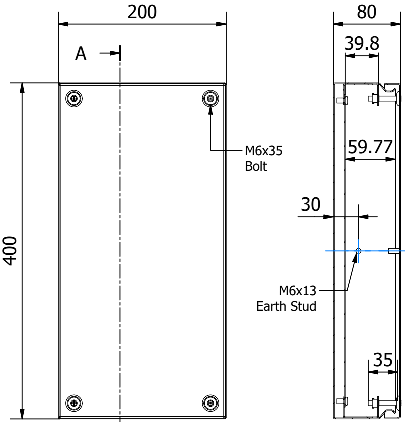
FRONT VIEW SECTION VIEW A-A
