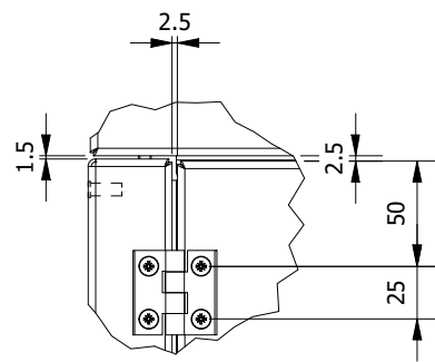
DETAIL C
