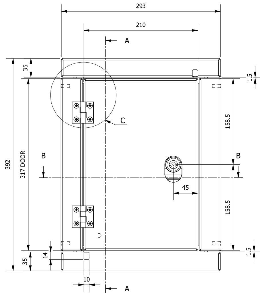
FRONT VIEW
